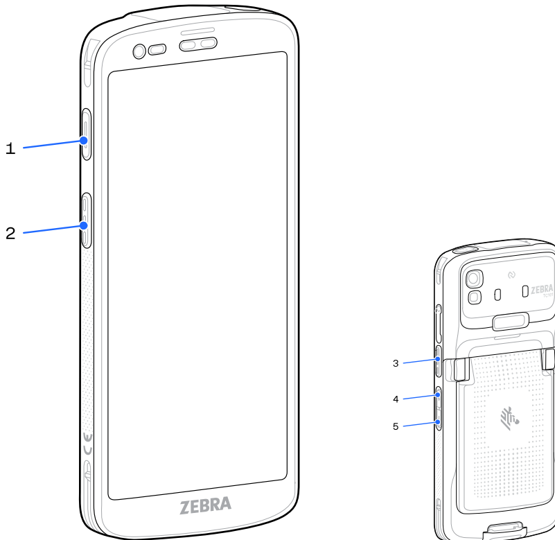
Figure 8 Button Positions
