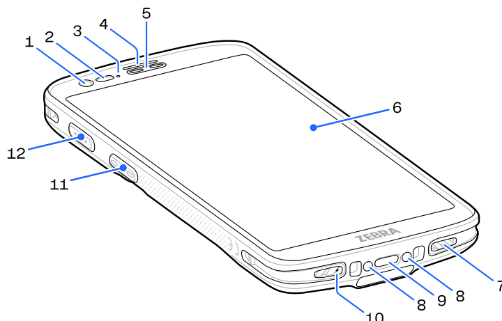
Figure1 Front View
