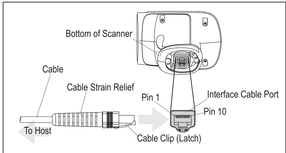
Figure 7. Standard Cable Pinouts
