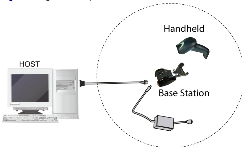
Figure 12. Single Reader Layout
