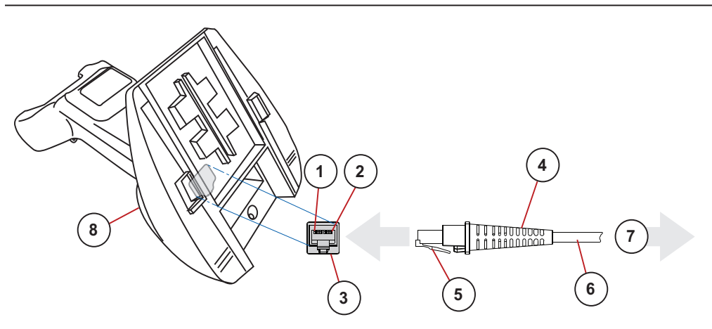
Figure 20. Standard Cable Pinouts: Base Station
