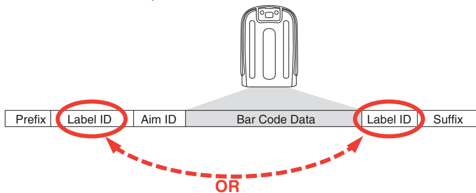
Figure 18. Label ID Position Options
