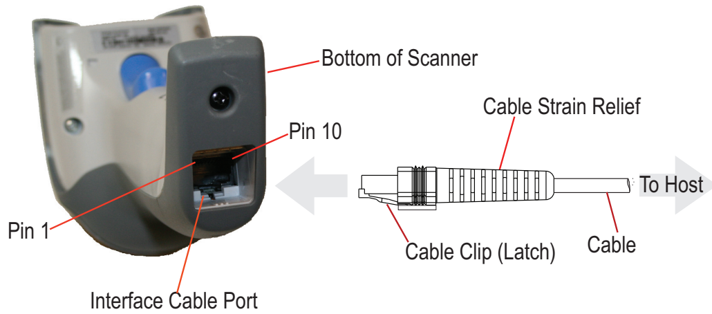
Figure 19. Standard Cable Pinouts: Handheld
