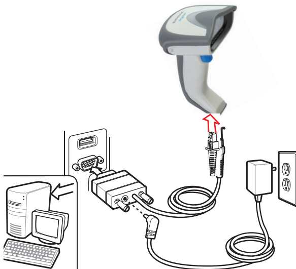
Figure 3. RS-232 Connection
